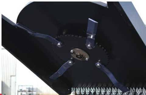
SERRATED 4-BLADE CARRIER
